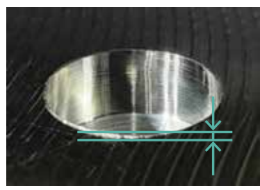
Cutting conditions: \phi 8.0 mm, 5xD, 42CrMo4, v_c = 90 m/min, f = 0.20 mm/rev, wet (internal supply)
