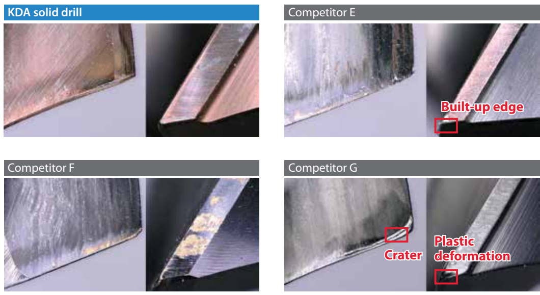
Cutting conditions: \phi 8.0 mm, 5xD, 42CrMo4, v_c = 90 m/min, f = 0.20 mm/rev, hole depth = 40 mm, wet (internal supply), 640 holes (36 m / 26 min.)
