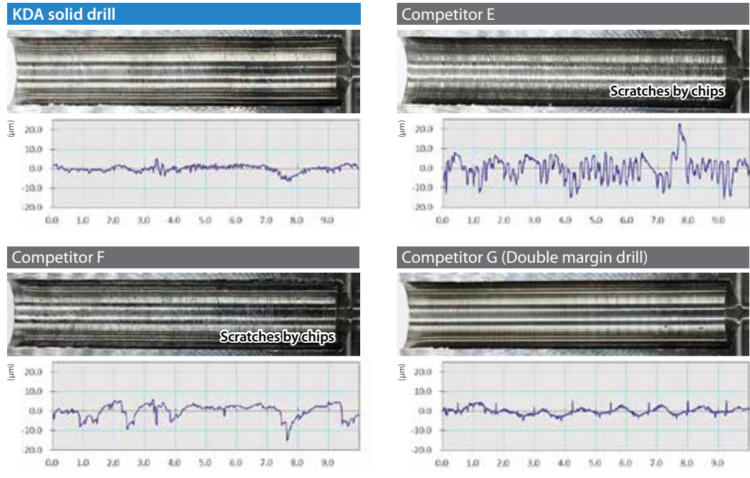
Cutting conditions: \phi 8.0 mm, 5xD, 42CrMo4, v_c = 90 m/min, f = 0.20 mm/rev, hole depth = 40 mm, wet (internal supply), 640 holes (36 m / 26 min.)
