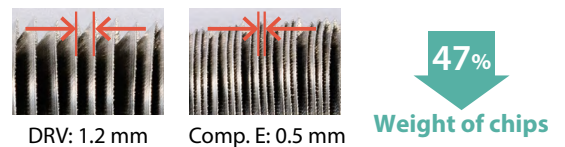
Pitch comparison of chips generated by the inner edge (In-house evaluation)
